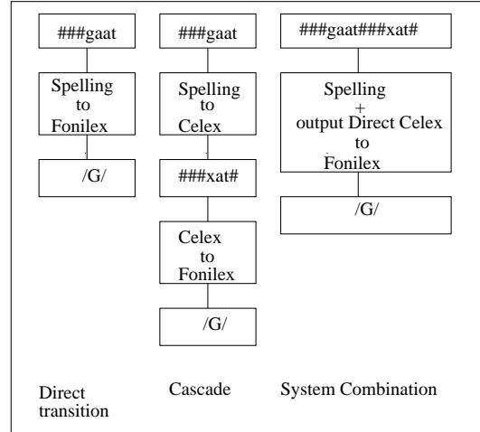
Figure 1. Architecture of three different approaches applied to the Fonilex phonemic transcription: training a single classifier on Fonilex, training a classifier for Fonilex using the predicted output for Celex as an additional information source in a cascade and in classifier combination.
