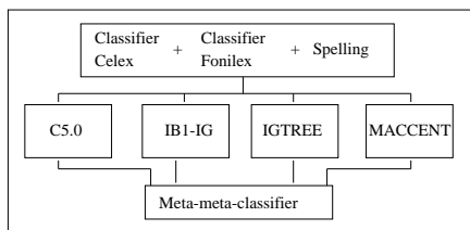
Figure 2. Architecture of the meta-meta-learning process. Component meta-classifiers are C5.0, IB1-IG, IGTREE, MACCENT
